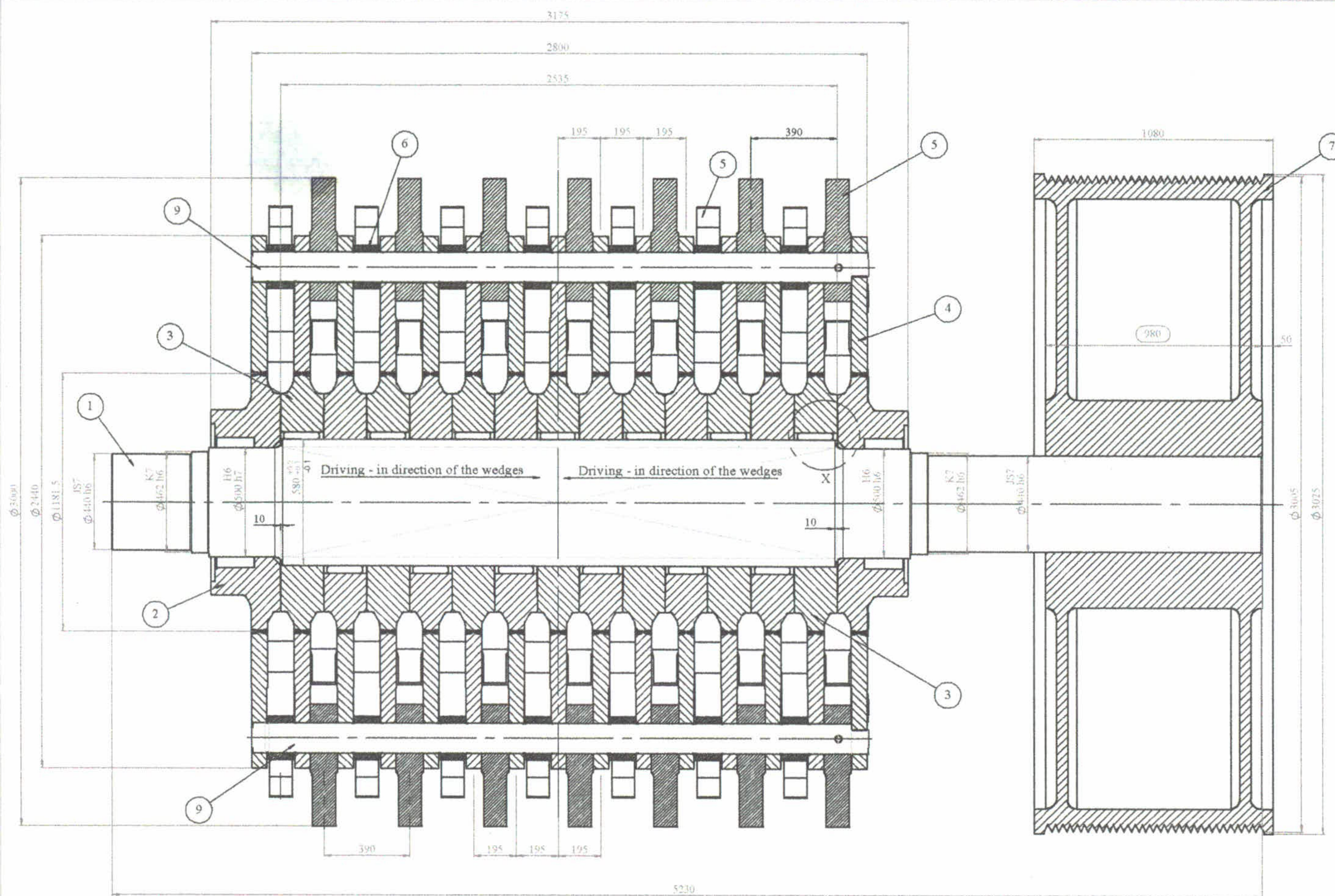
SECTION B-B
