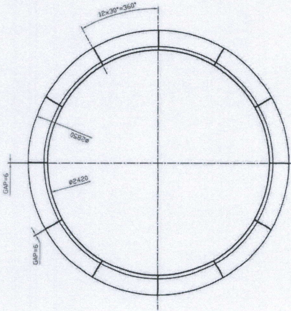
assembly view
