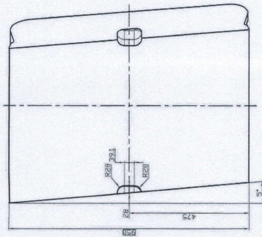
VIEW N
