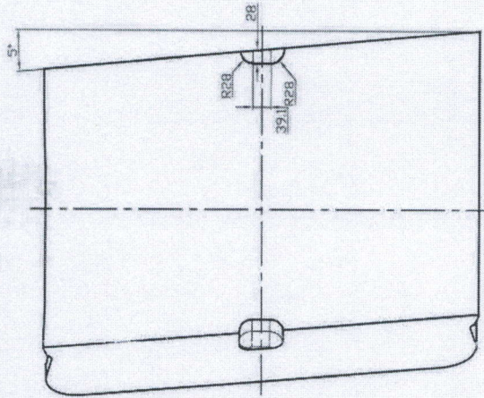
VIEW G
