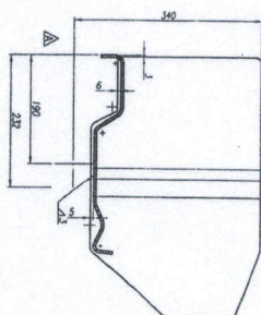
SECTION A-A (Type B) SCALE 1:5
