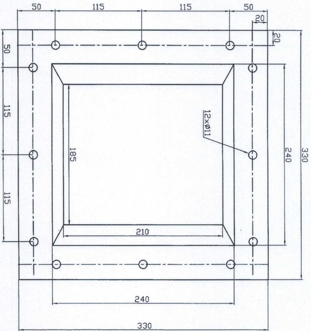
VIEW M
