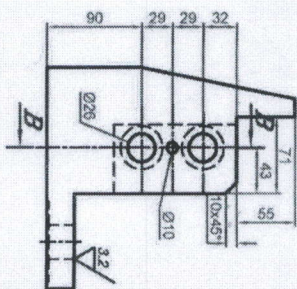
VIEW M
