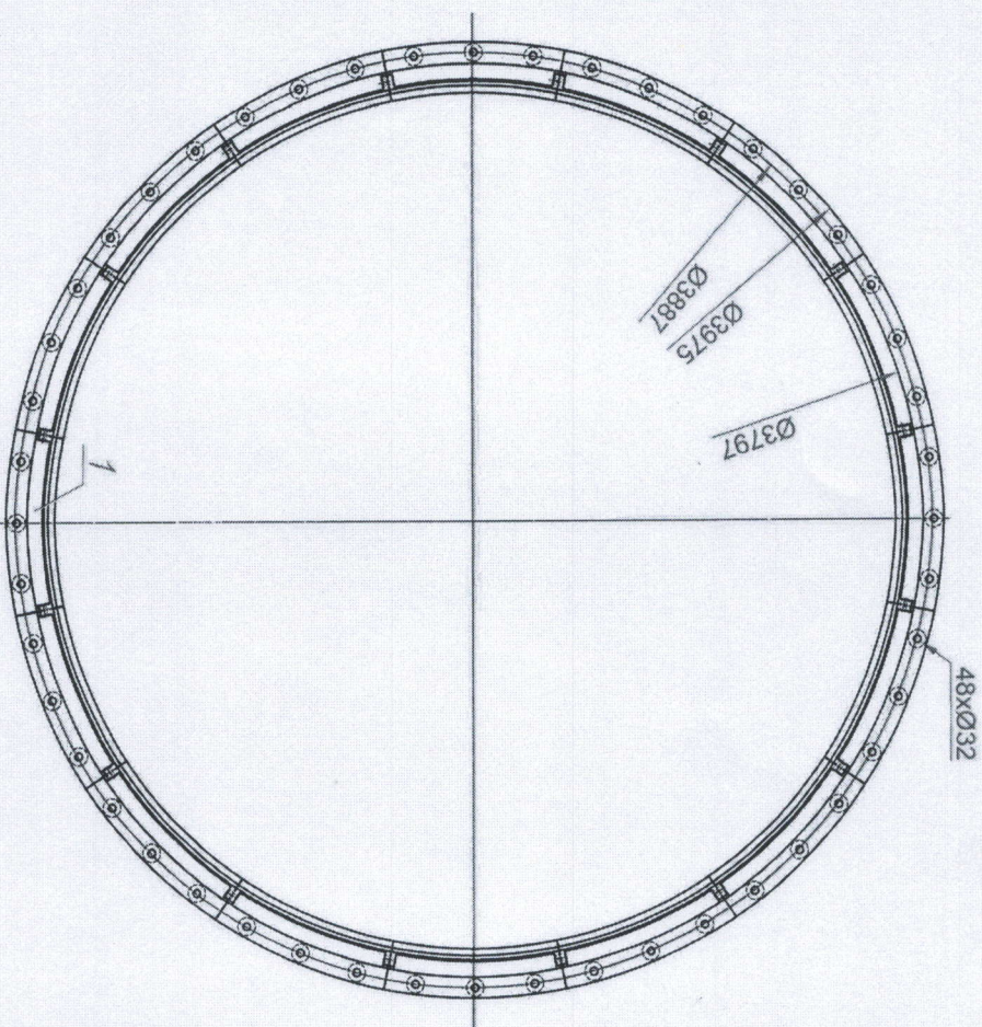
assembly view
